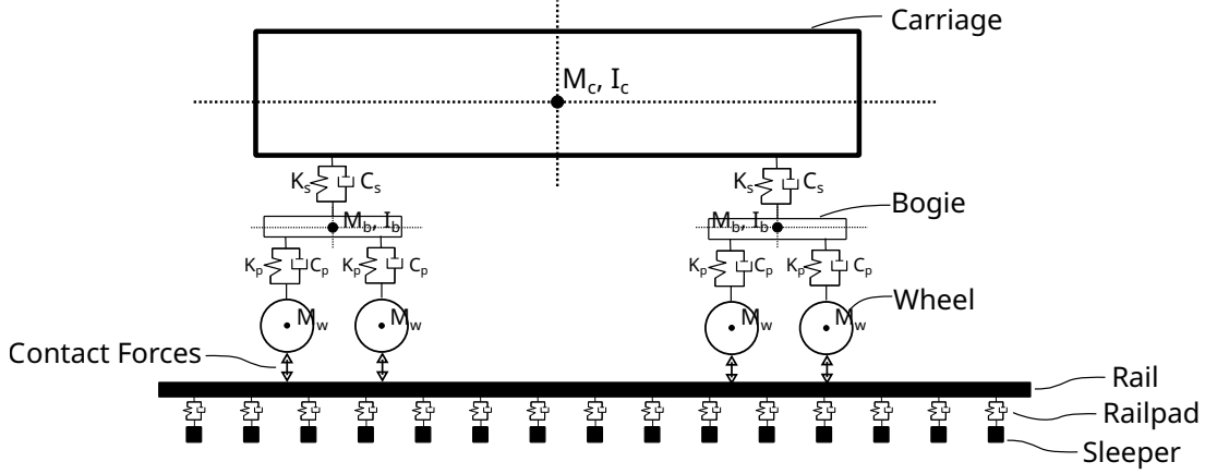
Figure 1: Schematic representation of the train–track interaction model. The sleepers are supported by spring–damper elements representing the ballast and subgrade, which may exhibit linear or piecewise-linear, and spatially varying (random), stiffness behaviour.
