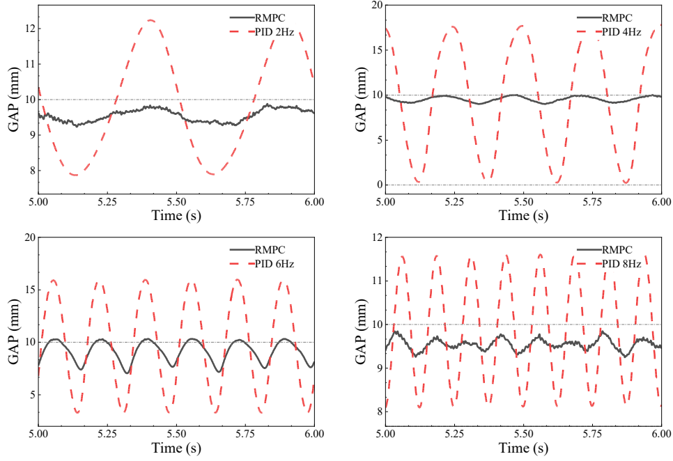
Figure 7 Harmonic aerodynamic load conditions co-simulation results
