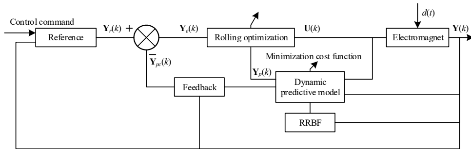
Figure 2 Schematic diagram of RMPC
