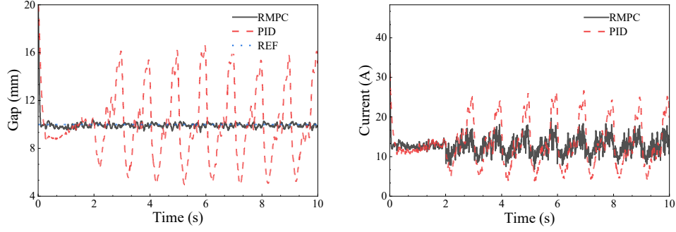
Figure 11 Non-stationary aerodynamic loads and random track irregularities co-simulation results
